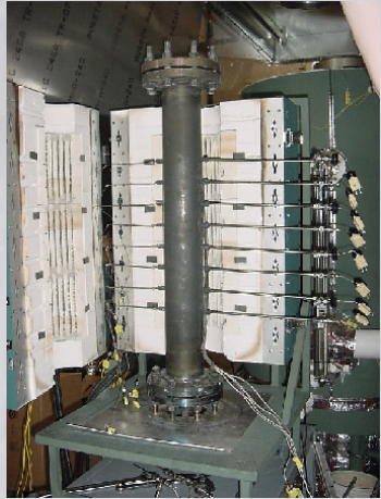
Sub-Scale furnace experiment
