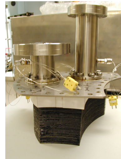
Plate Stack attached to Reforming side Manifold
