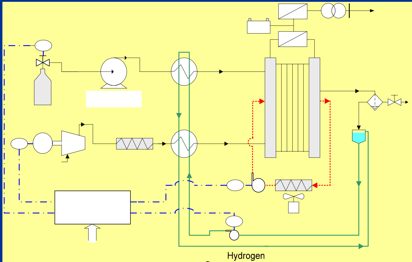
PEM fuel cell system block diagram that shows the auxiliary components along with input and output signals.
