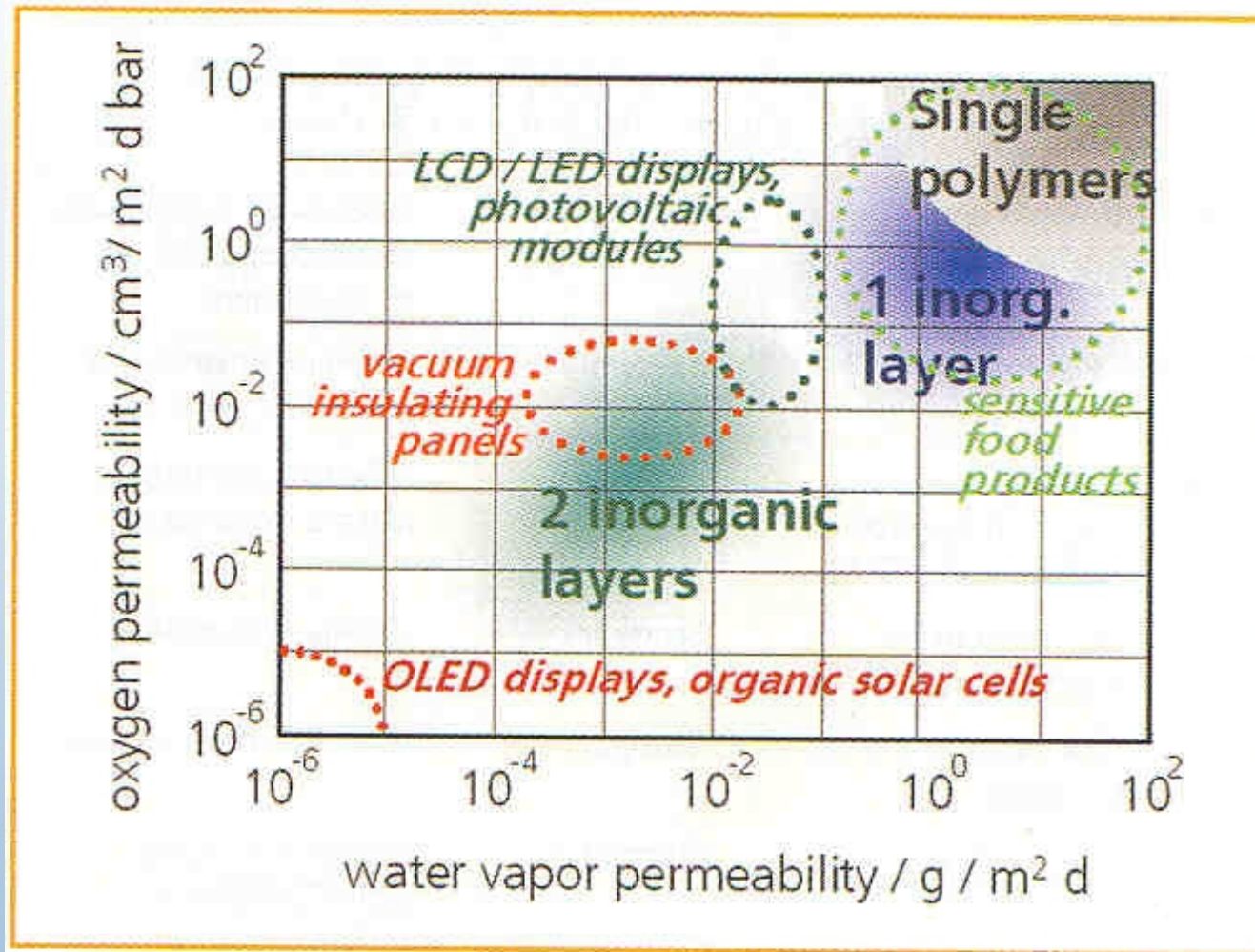
Figure 1. Barrier requirements for different product sectors (dotted lines, italics) and performance of flexible polymeric structures (shaded areas) [1].
